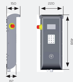
Terminal a mural
